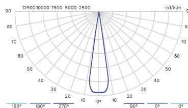
7051 Light Beam 17°
